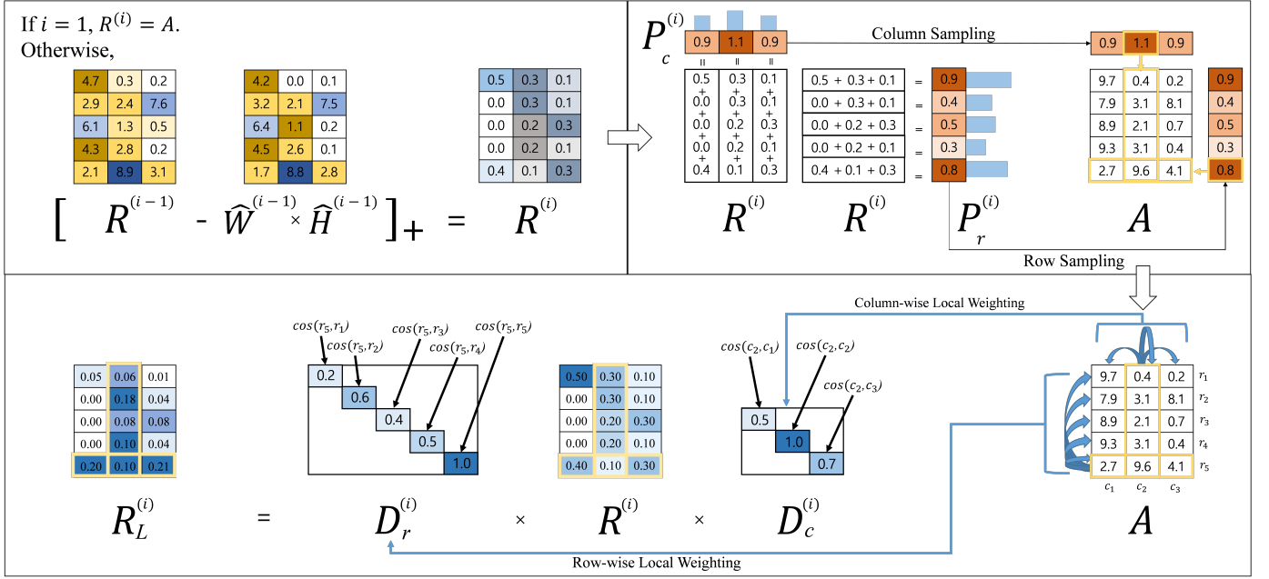
Fig. 2: Overview of the proposed ensemble approach
